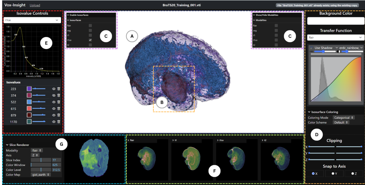
Figure 1: The Vox-Insight framework, shown here with a multimodal brain MRI from the BraTS20 dataset. (A) is the rendered 3D view with (B) tumor highlighted, (C) controls which modalities are shown in the volume renderer, and (D) provides per-modality coloring and clipping controls; (E) cumulative Laplacian histogram, computed for each modality. Prominent peaks mark candidate isovalues; each can be toggled, re-colored, or re-weighted; the histogram also allows the selection of new isovalues. (F) for every modality the X-, Y- and Z-direction gradient magnitudes are collapsed to 2-D heat-maps, providing a quick visual summary of edge content; (G) 2-D renderer for axial, coronal, or sagittal slices of any modality with independent window/level and color map controls.
